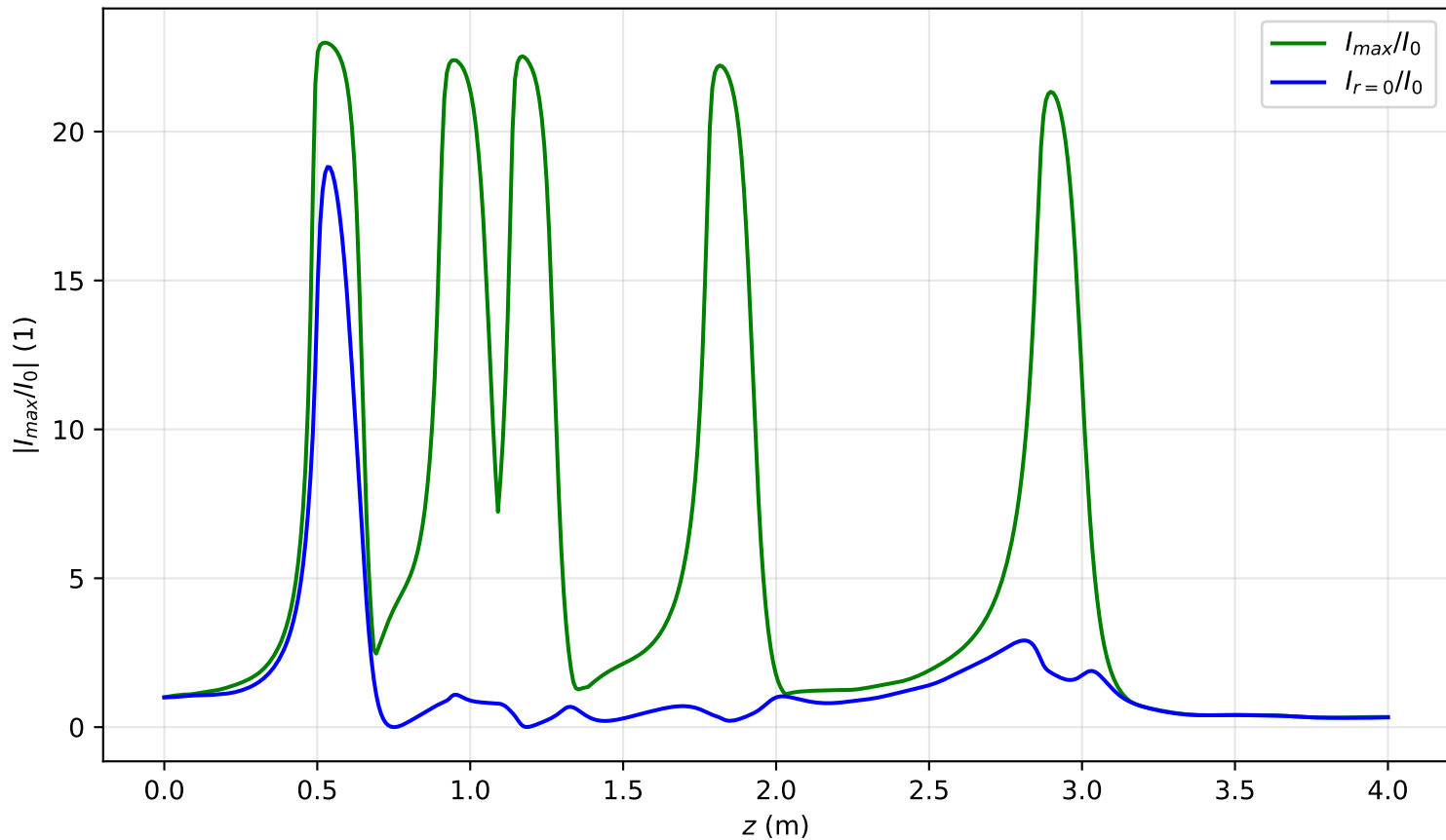
I_{max}(x=0, y=0, z)/I_0 , P_{in}=4.8P_{cr} , noisy input, artificial time
